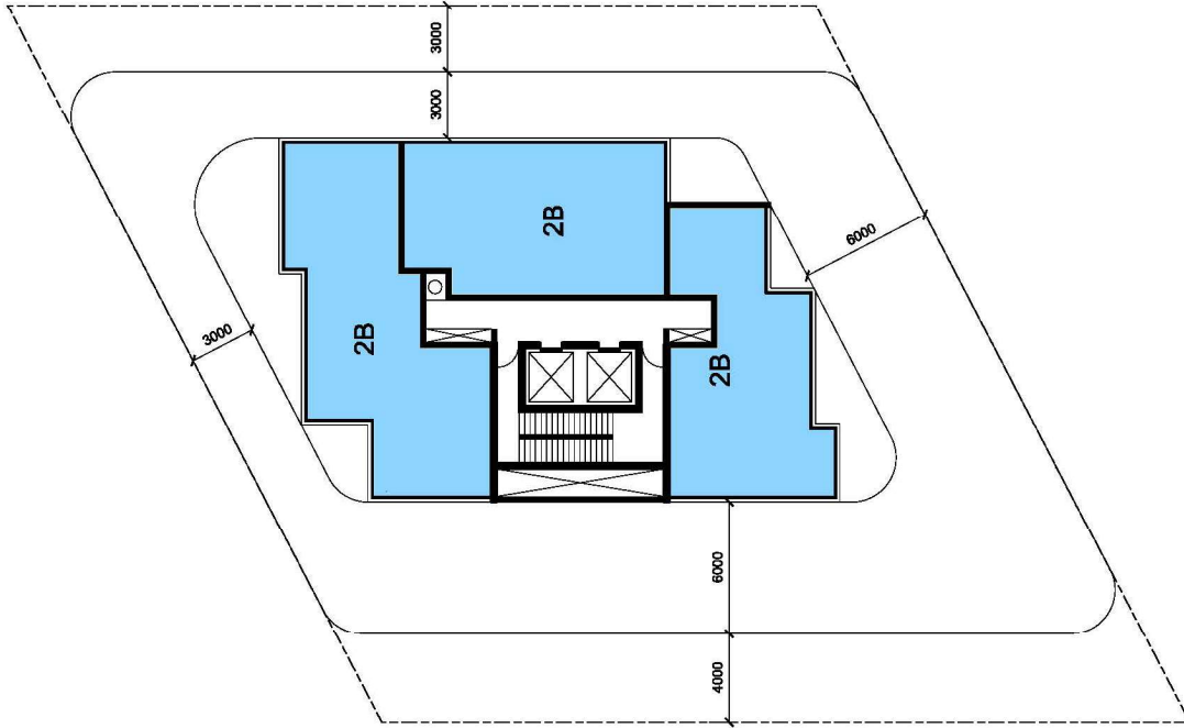
1 TYPICAL FLOOR PLAN L15-L25, Plant Room On L14
